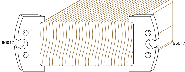
Rounded double, 48mm radius 3
