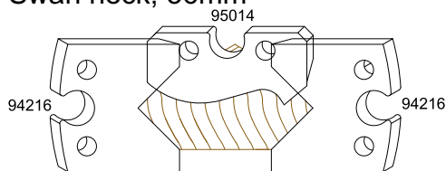
Swan neck, 56mm
