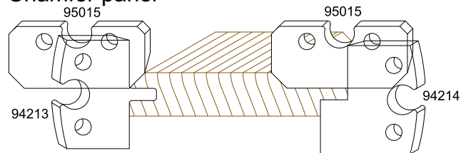
Double 45deg Chamfer panel
