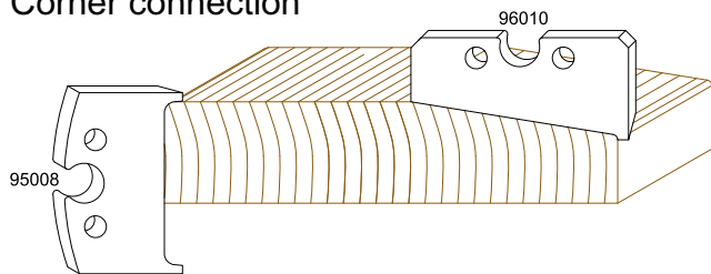
Corner connection
