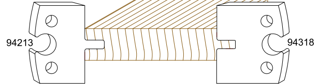
Tongue & groove 4,5mm
