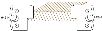
Loghouse panel, 45mm
