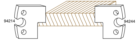
Loghouse panel, 70mm
