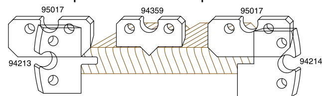
Chamfer panel with middle profile
