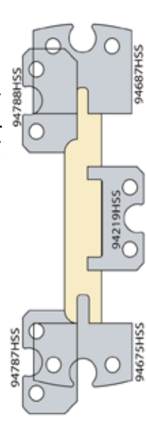
Double rounded T&G (open)
