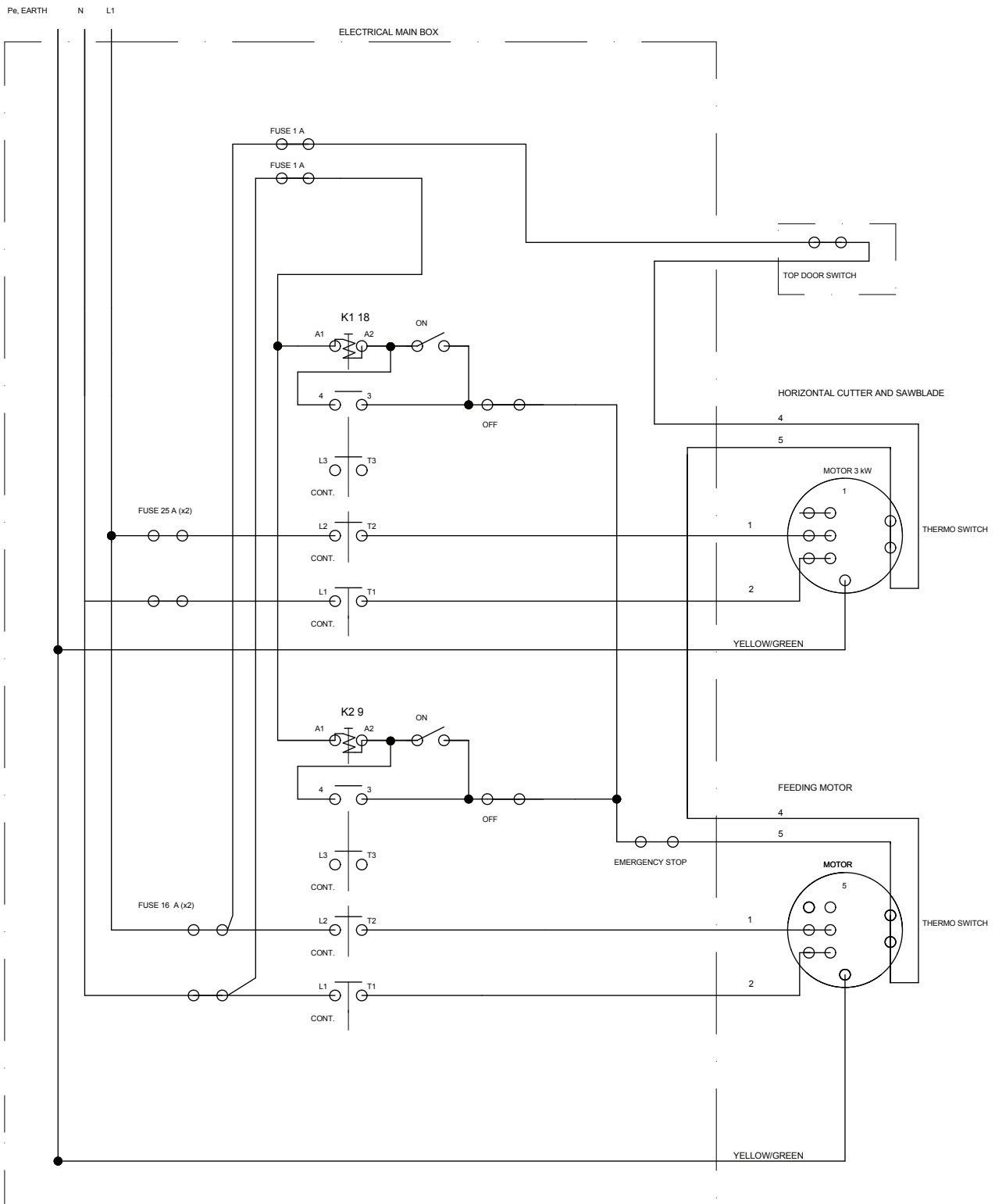
ELECTRICAL DRAWING SH410, 230 VOLT 1-PHASE, EU
